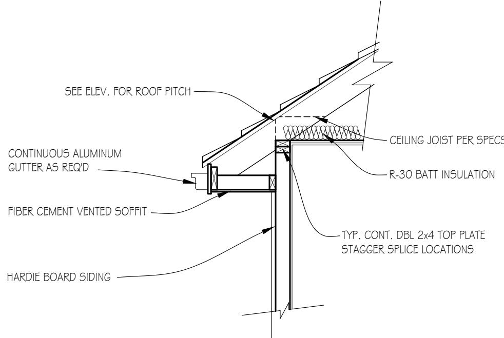
DETAIL: ROOF FRAMED ON TOP OF PLATE NOT TO SCALE
