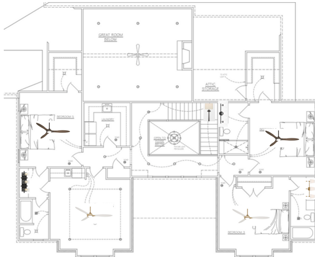
ELECTRICAL PLAN SECOND FLOOR
