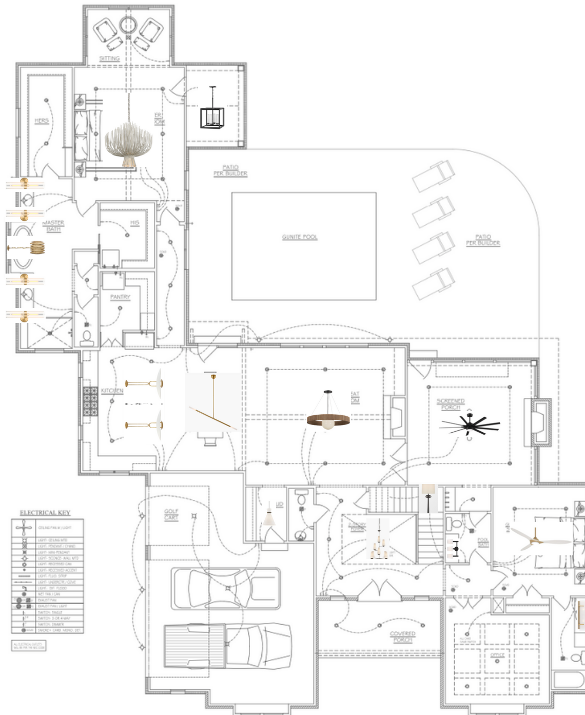
ELECTRICAL PLAN FIRST FLOOR
